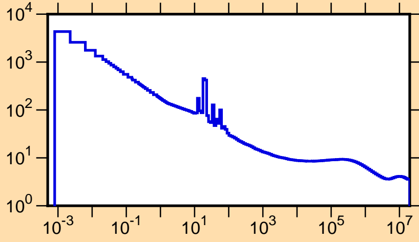
\sigma vs. E for ^{89}\text{Mo}(n,\text{tot.})
