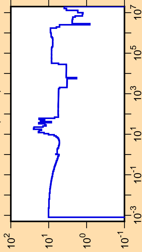
\Delta\sigma/\sigma vs. E for ^{89}\text{Mo}(n,\text{tot.})
