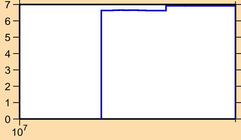
\Delta\sigma/\sigma vs. E for ^{90}\text{Mo}(n,\text{nonel.})
