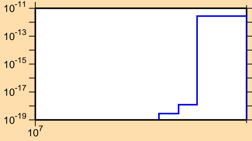
\sigma vs. E for ^{90}\text{Mo}(n,\text{pt})
