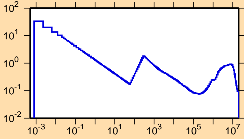
\sigma vs. E for ^{90}\text{Mo}(n,p)
