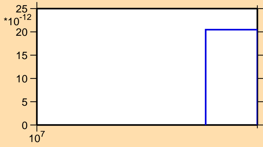
\sigma vs. E for ^{90}\text{Mo}(n,\text{nd})
