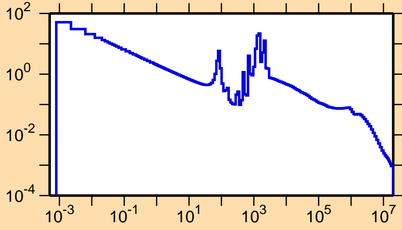
\sigma vs. E for ^{90}\text{Mo}(n,\gamma)
