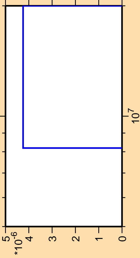
\Delta\sigma/\sigma vs. E for ^{90}\text{Mo}(n,2np)
