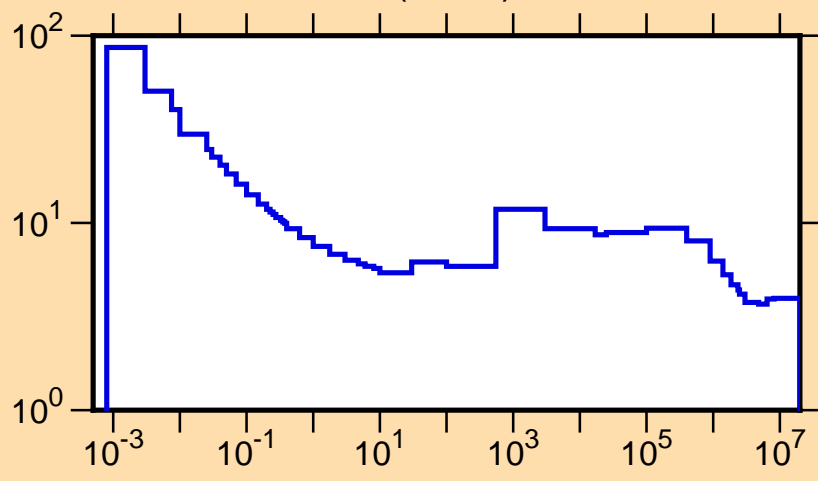
\sigma vs. E for ^{90}\text{Mo}(n,\text{tot.})
