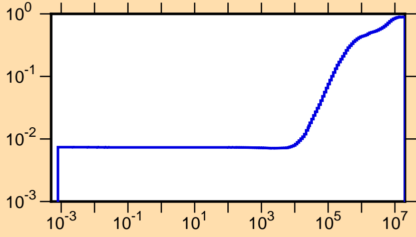
\mu vs. E for ^{91}\text{Mo}(\text{mt251})
