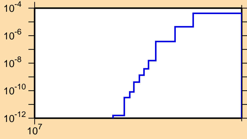
\sigma vs. E for ^{91}\text{Mo}(n,pd)
