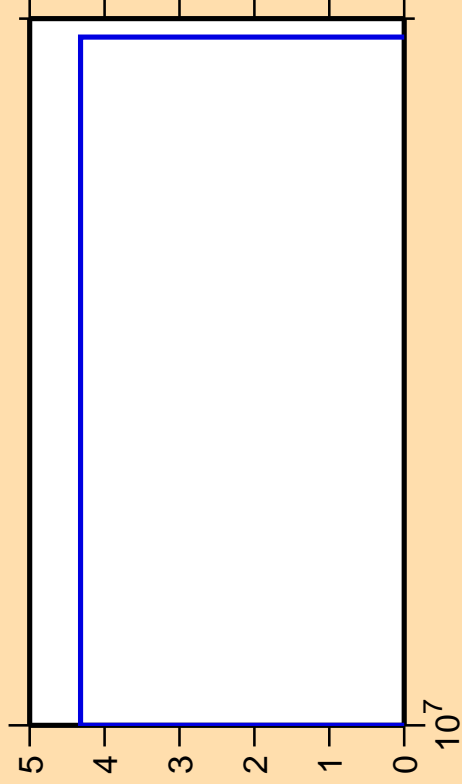
\Delta\sigma/\sigma vs. E for ^{91}\text{Mo}(n,n\text{cont.})
