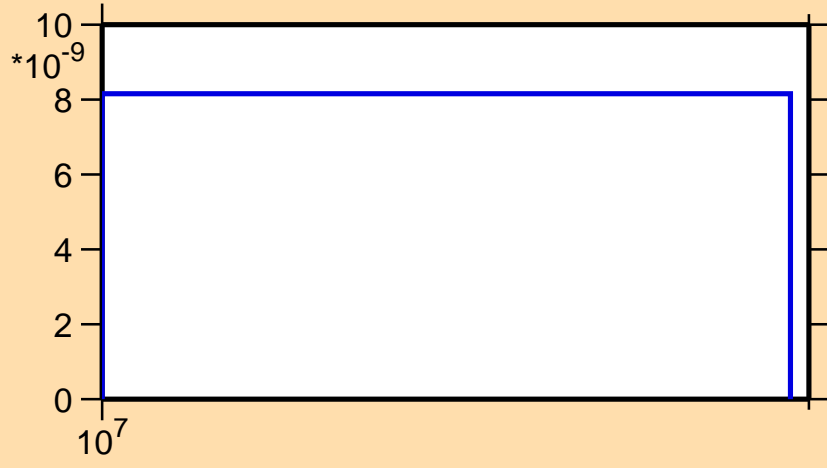
\sigma vs. E for ^{91}\text{Mo}(n,nd)
