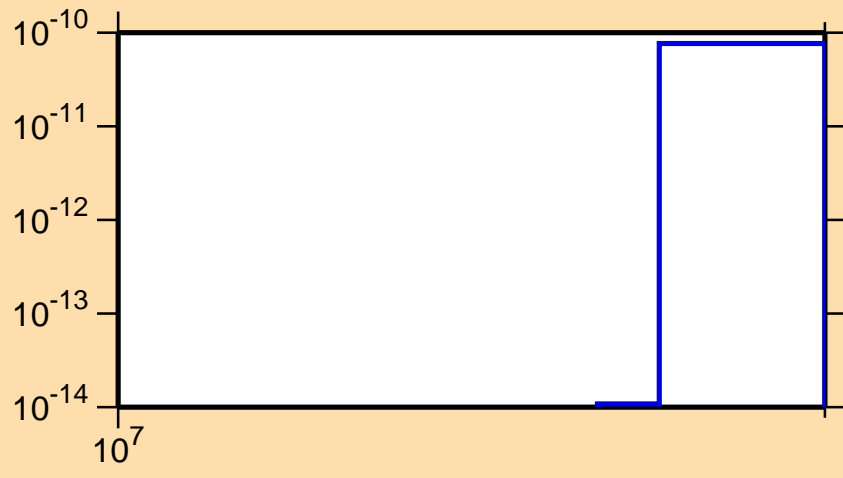
\sigma vs. E for ^{91}\text{Mo}(\text{mt } 34)
