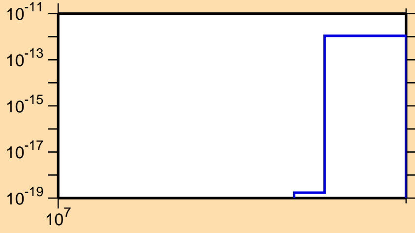
\sigma vs. E for ^{91}\text{Mo} (mt 45)
