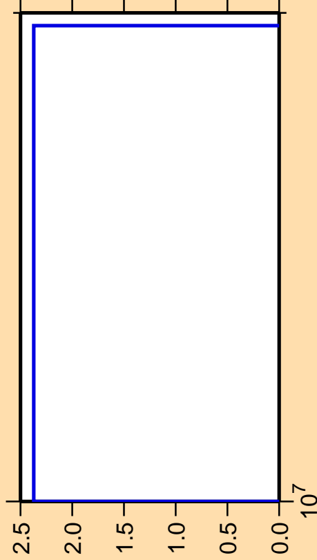
\Delta\sigma/\sigma vs. E for ^{91}\text{Mo}(\text{mt } 34)
