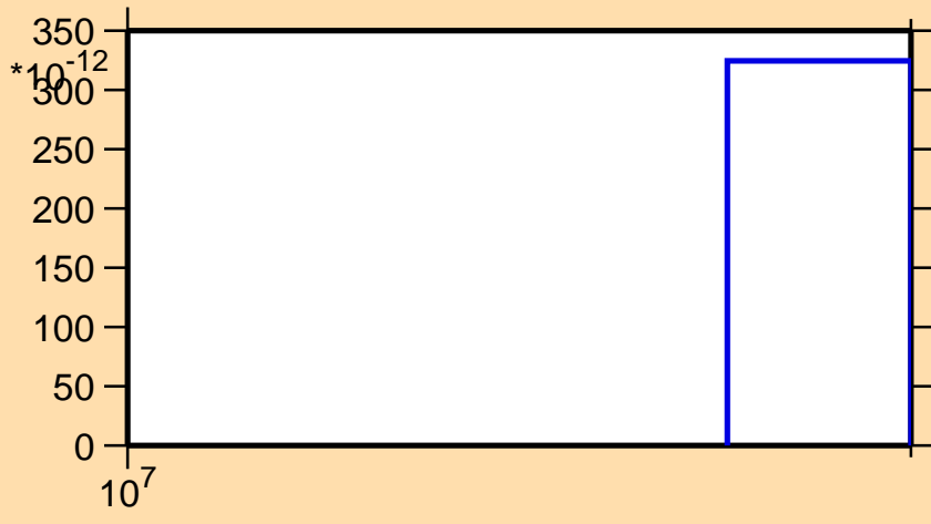
\sigma vs. E for ^{92}\text{Mo}(n,\text{nd})
