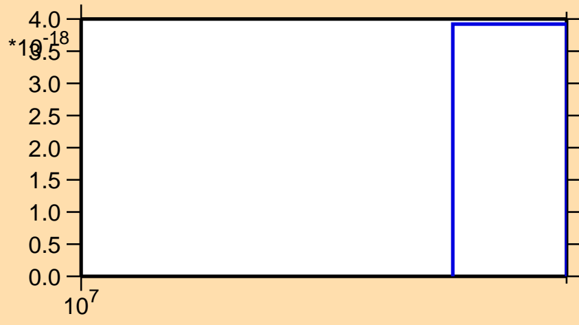
\sigma vs. E for ^{92}\text{Mo}(n,2np)
