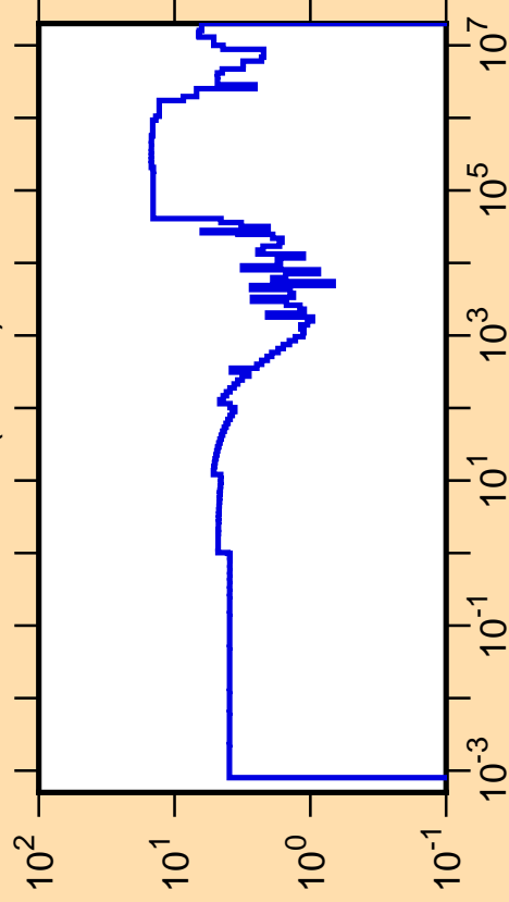
\Delta\sigma/\sigma vs. E for ^{92}\text{Mo}(n,\text{tot.})
