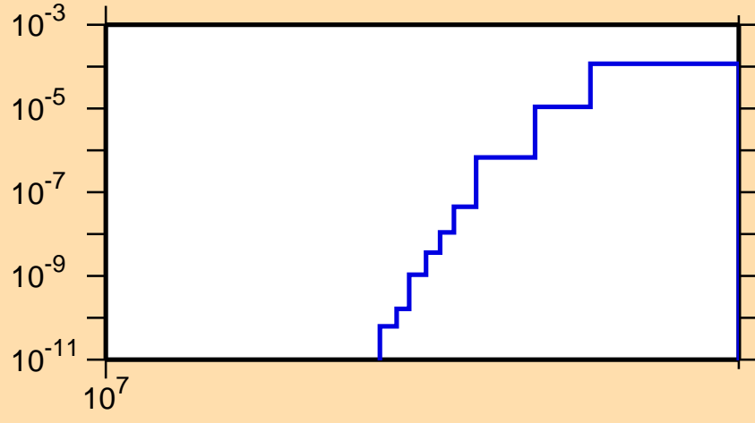
\sigma vs. E for ^{92}\text{Mo}(n,t)
