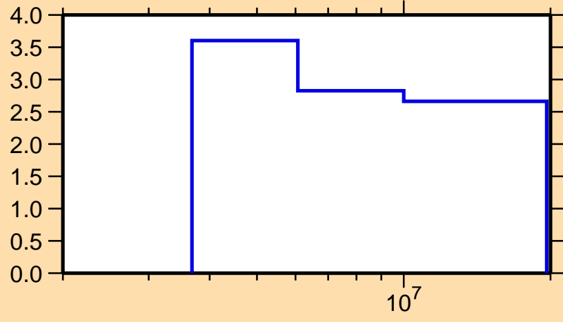
\Delta\sigma/\sigma vs. E for ^{92}\text{Mo}(n,n\text{onel.})
