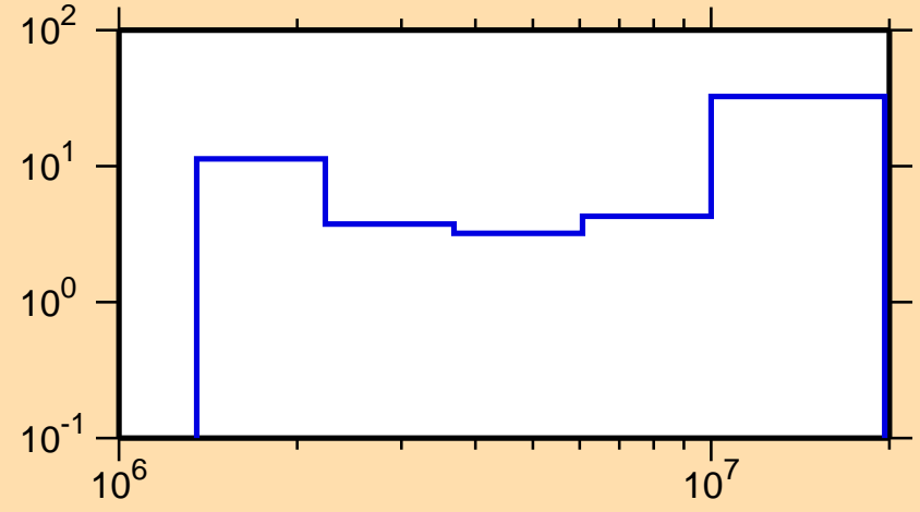
\Delta\sigma/\sigma vs. E for ^{92}\text{Mo}(n,\text{inel.})
