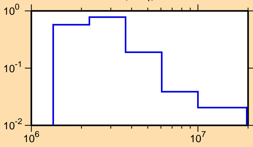
\sigma vs. E for ^{92}\text{Mo}(n,n_1)
