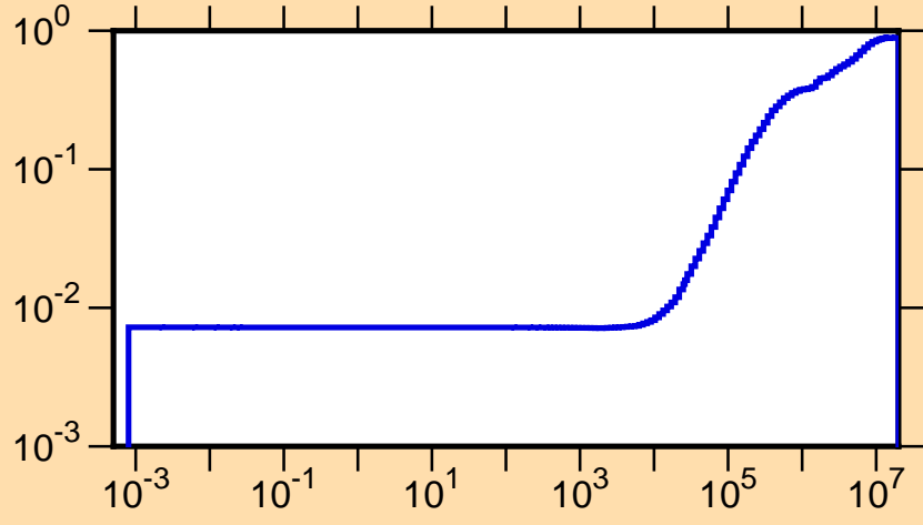
\mu vs. E for ^{93}\text{Mo}(\text{mt251})
