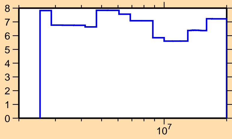
\Delta\sigma/\sigma vs. E for ^{93}\text{Mo}(n,n\text{nonel.})
