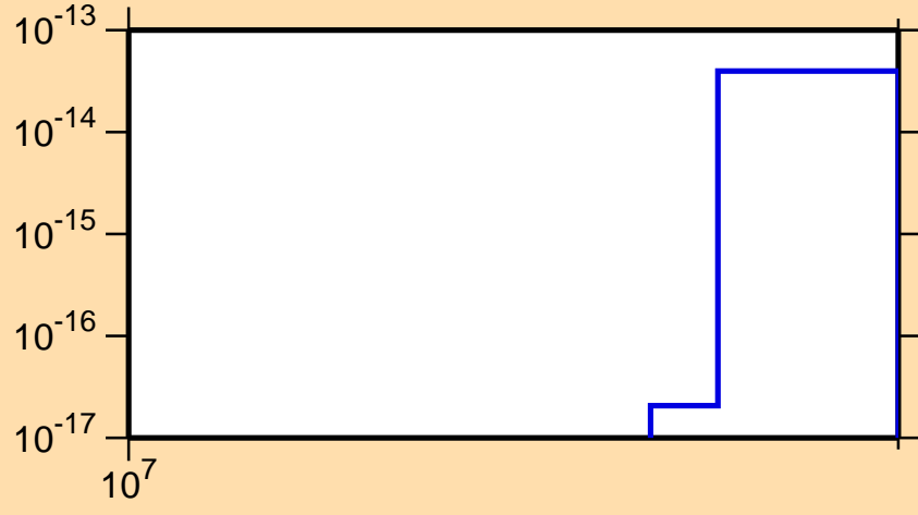
\sigma vs. E for ^{93}\text{Mo} (mt 45)
