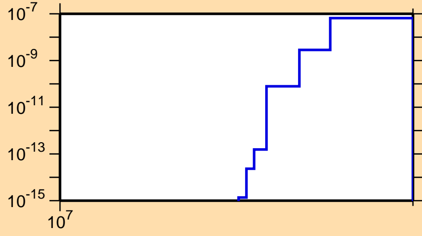
\sigma vs. E for ^{93}\text{Mo}(n,pd)
