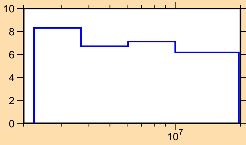
\Delta\sigma/\sigma vs. E for ^{93}\text{Mo}(n,n\text{inel.})
