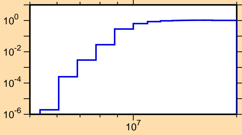
\sigma vs. E for ^{93}\text{Mo}(n,2n)
