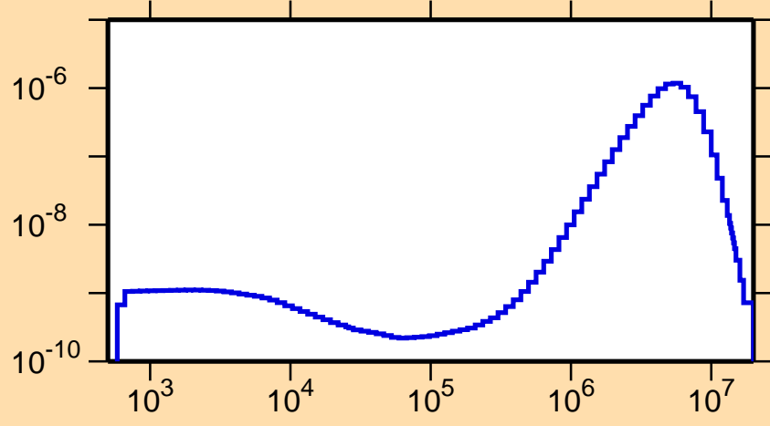
\sigma vs. E for ^{93}\text{Mo}(n,n_2)
