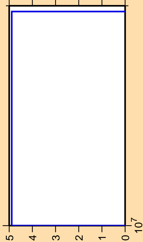
\Delta\sigma/\sigma vs. E for ^{93}\text{Mo} (mt 45)
