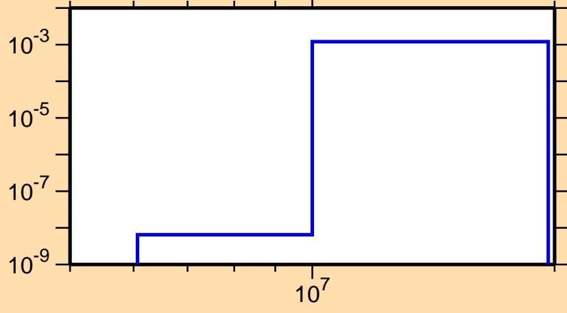
\sigma vs. E for ^{93}\text{Mo}(n,t)
