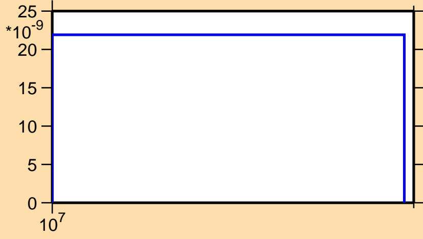
\sigma vs. E for ^{93}\text{Mo}(n,\text{pt})
