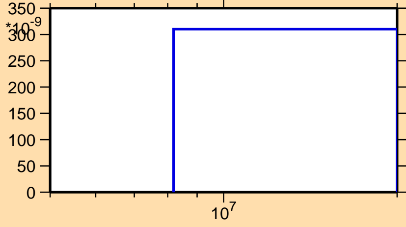
\sigma vs. E for ^{93}\text{Mo}(n,3n)
