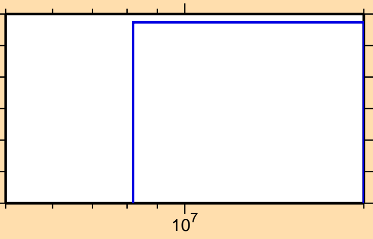
\sigma vs. E for ^{93}\text{Mo}(n,2np)
