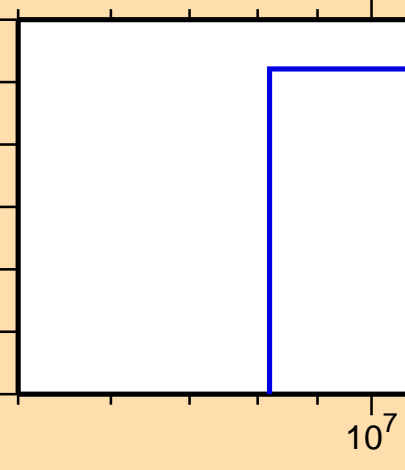
\sigma vs. E for ^{93}\text{Mo} (mt 45)
