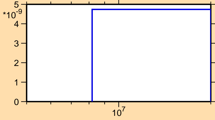
\sigma vs. E for ^{93}\text{Mo}(n,\text{pd})
