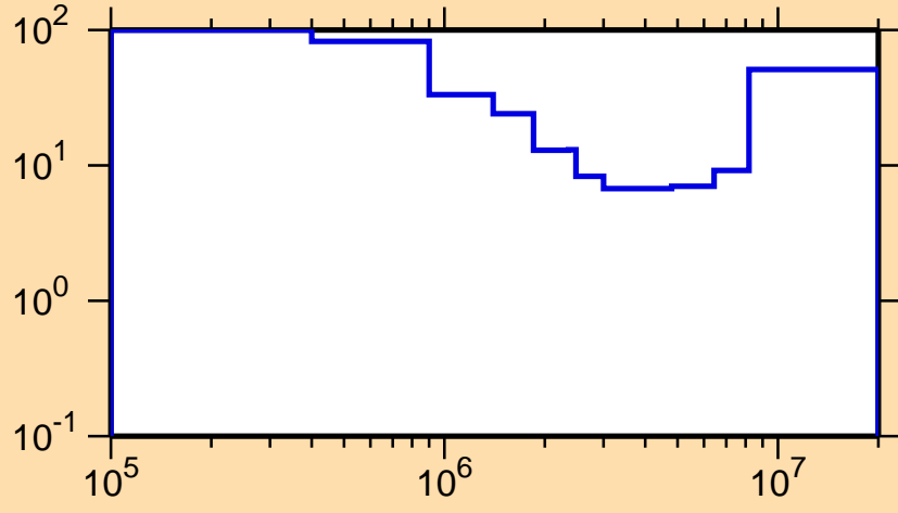
\Delta\sigma/\sigma vs. E for ^{93}\text{Mo}(n,n\text{cont.})
