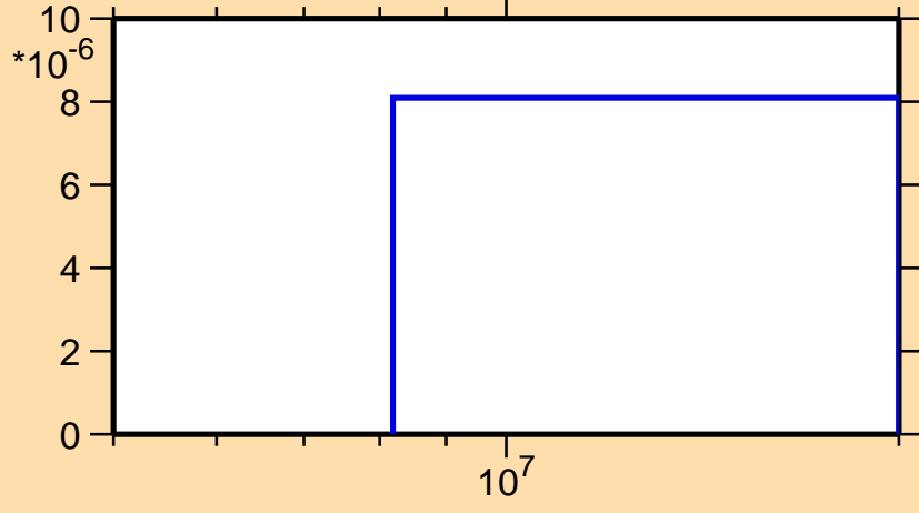
\sigma vs. E for ^{93}\text{Mo}(n,\text{nd})
