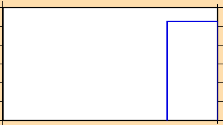
\sigma vs. E for ^{95}\text{Mo}(n,3n)
