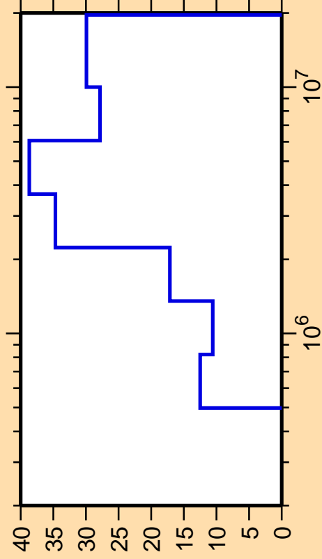
\Delta\sigma/\sigma vs. E for ^{95}\text{Mo}(n,n_3)
