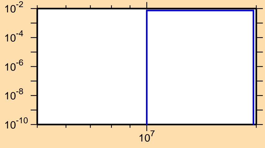
\sigma vs. E for ^{95}\text{Mo}(n,np)
