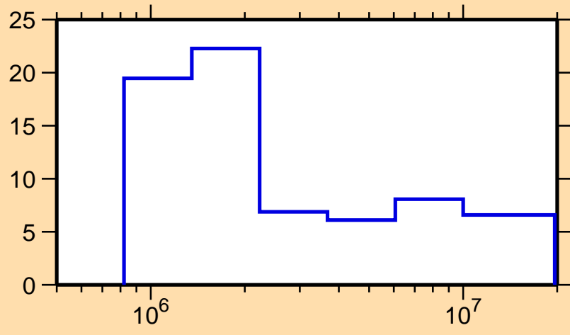
\Delta\sigma/\sigma vs. E for ^{95}\text{Mo}(n,el.)
