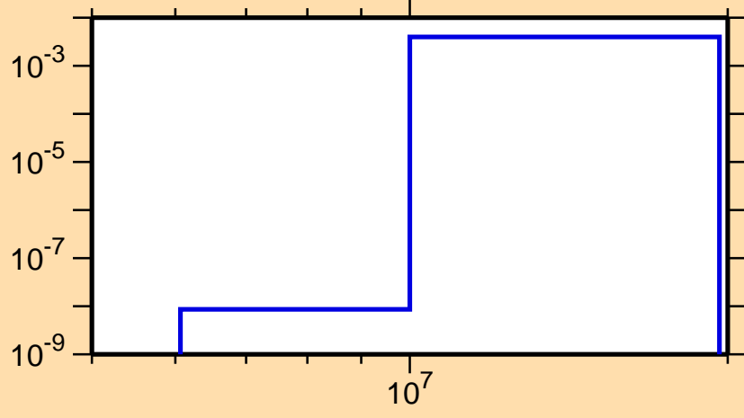
\sigma vs. E for ^{95}\text{Mo}(n,d)
