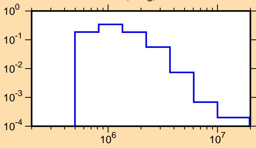
\sigma vs. E for ^{95}\text{Mo}(n,n_3)
