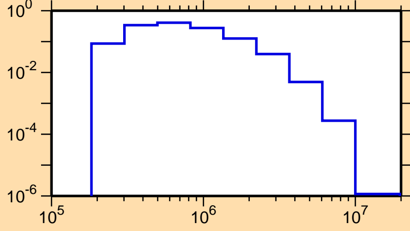
\sigma vs. E for ^{95}\text{Mo}(n,n_2)
