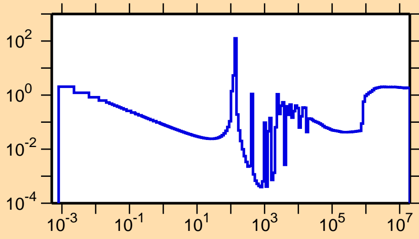
\sigma vs. E for ^{96}\text{Mo}(n,\text{nonel.})
