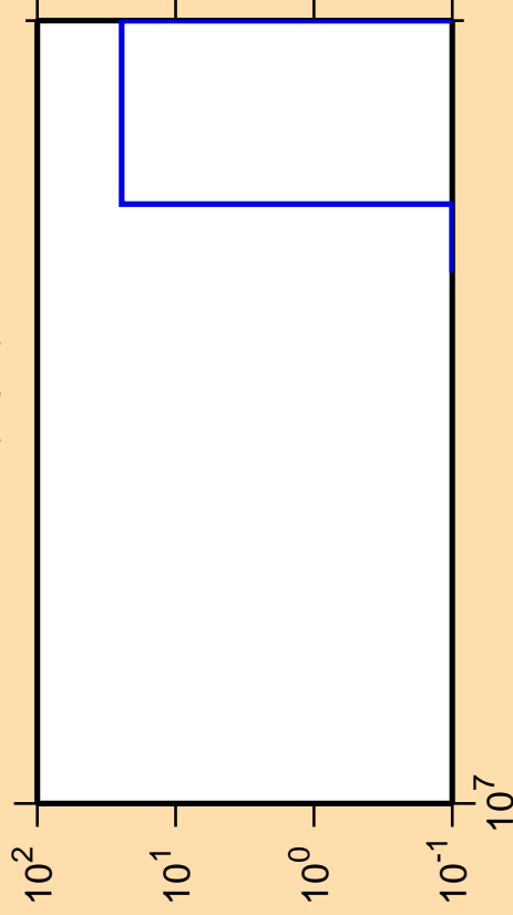
\Delta\sigma/\sigma vs. E for ^{96}\text{Mo}(n,\text{pd})
