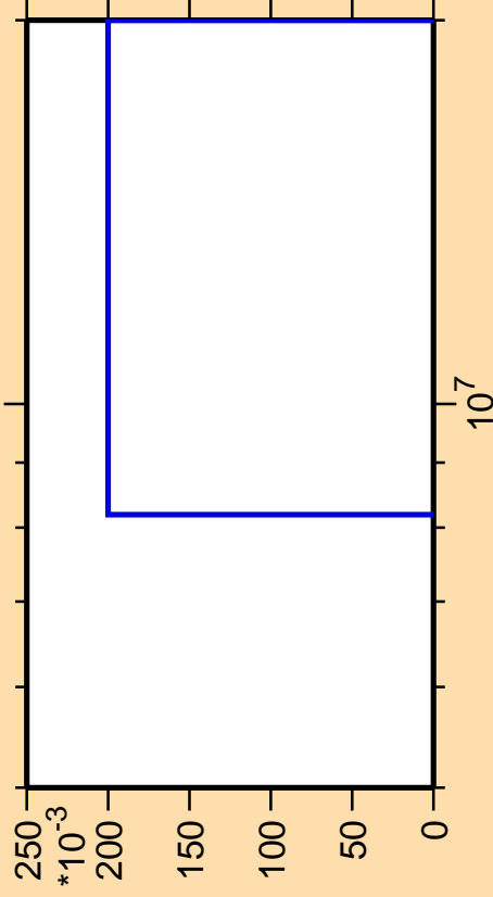
\Delta\sigma/\sigma vs. E for ^{96}\text{Mo}(n,pd)
