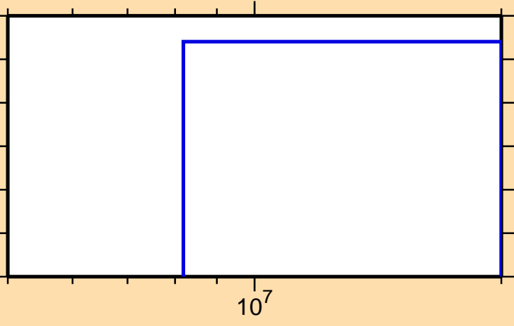
\sigma vs. E for ^{96}\text{Mo}(n,2n\alpha)
