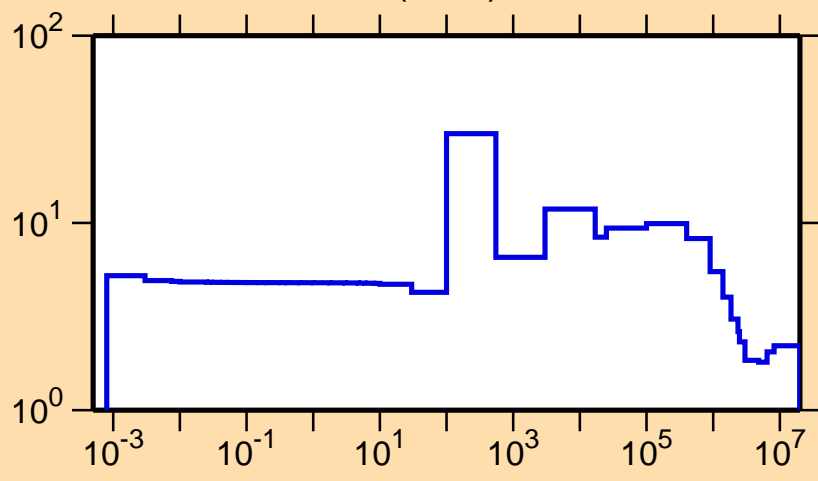
\sigma vs. E for ^{96}\text{Mo}(n,\text{el.})
