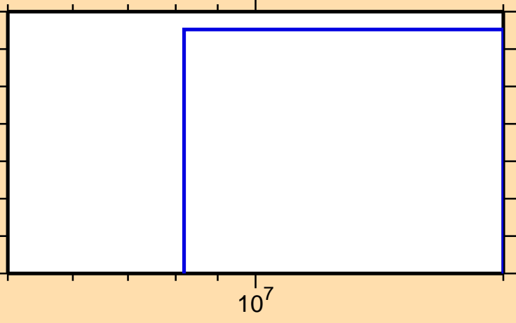
\sigma vs. E for ^{96}\text{Mo}(n,2np)
