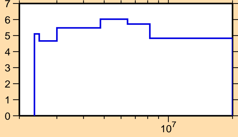
\Delta\sigma/\sigma vs. E for ^{96}\text{Mo}(n,\text{nonel.})
