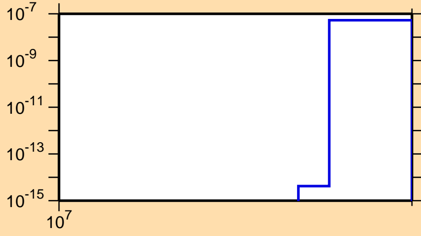
\sigma vs. E for ^{98}\text{Mo}(n,\text{nd})
