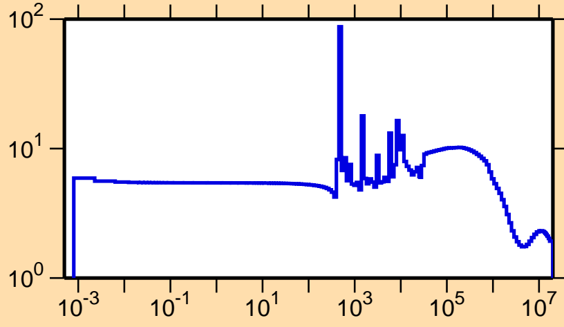
\sigma vs. E for ^{98}\text{Mo}(n,\text{el.})
