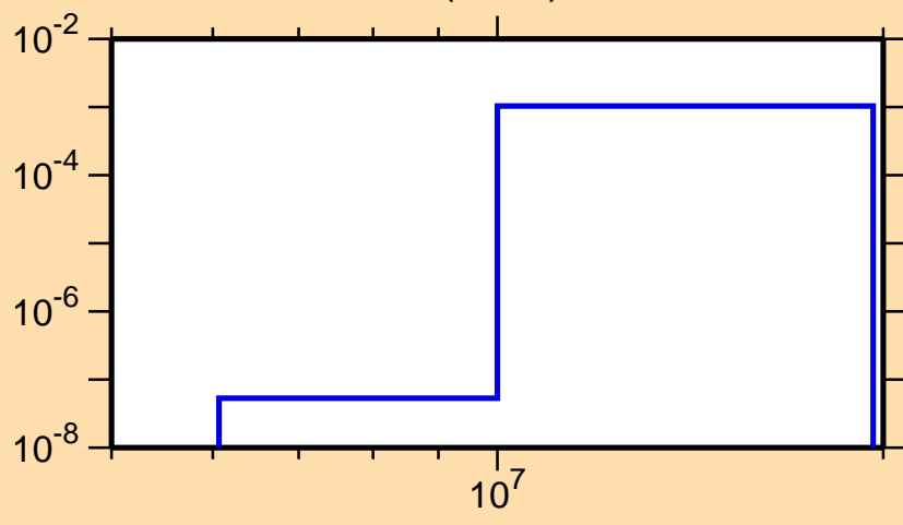
\sigma vs. E for ^{98}\text{Mo}(n,n\alpha)
