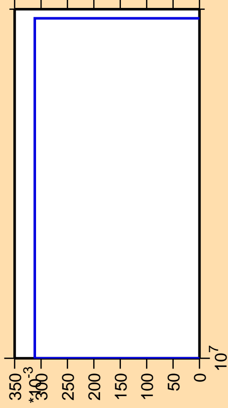
\Delta\sigma/\sigma vs. E for ^{98}\text{Mo}(n,2np)
