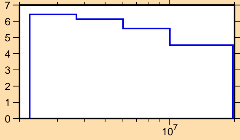
\Delta\sigma/\sigma vs. E for ^{98}\text{Mo}(n,n\text{onel.})
