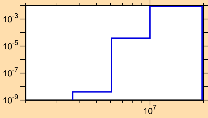
\sigma vs. E for ^{98}\text{Mo}(n,p)
