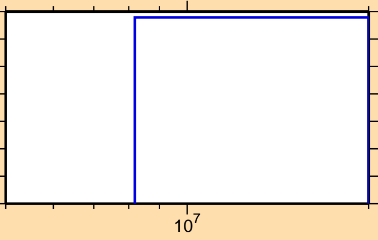
\sigma vs. E for ^{98}\text{Mo}(n,2n\alpha)
