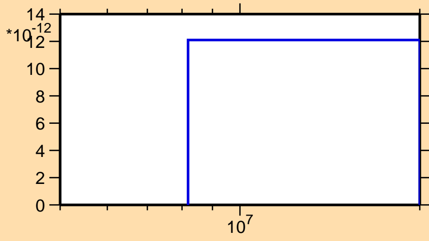
\sigma vs. E for ^{98}\text{Mo}(n,nt)
