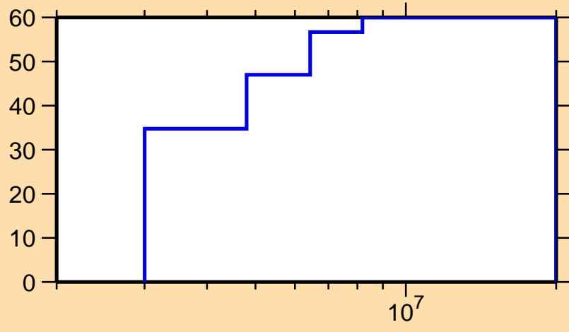
\Delta\sigma/\sigma vs. E for ^{98}\text{Mo}(n,n_1)
