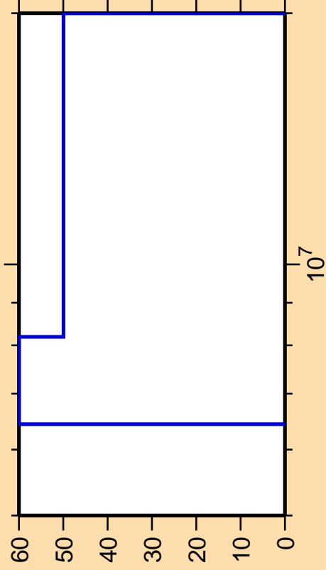
\Delta\sigma/\sigma vs. E for ^{98}\text{Mo}(n,n\alpha)
