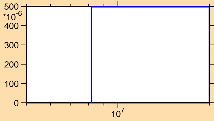
\sigma vs. E for ^{98}\text{Mo}(n,d)
