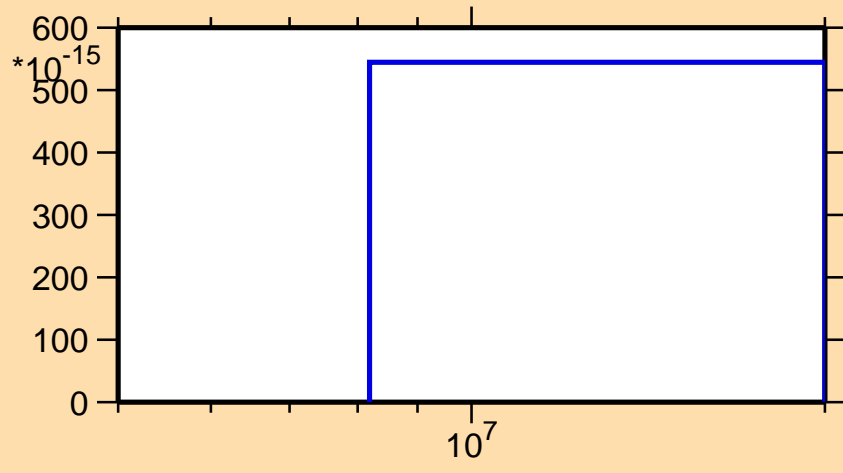
\sigma vs. E for ^{98}\text{Mo}(n,2np)
