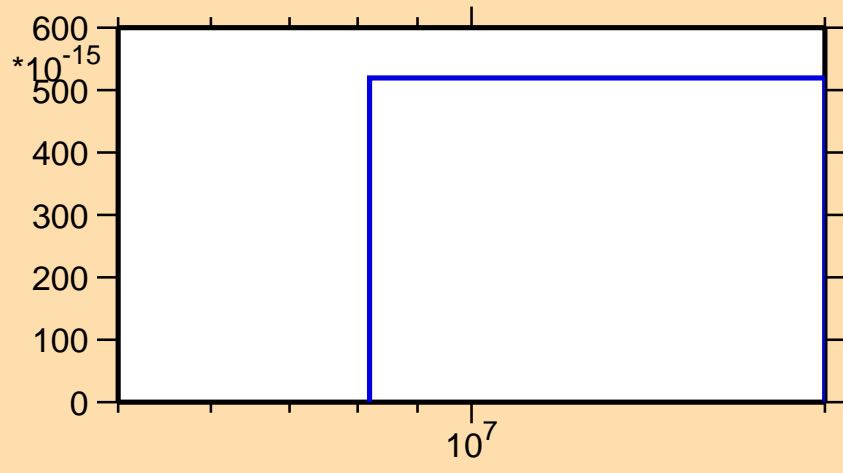
\sigma vs. E for ^{98}\text{Mo}(n,p\alpha)
