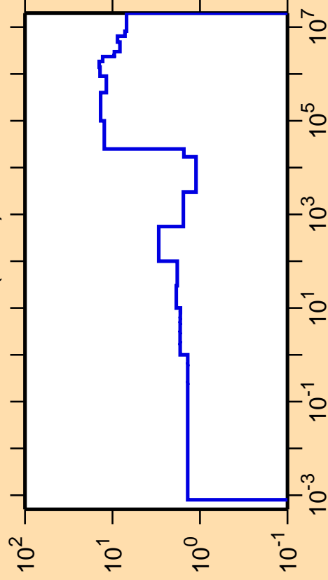
\Delta\sigma/\sigma vs. E for ^{98}\text{Mo}(n,\text{el.})
