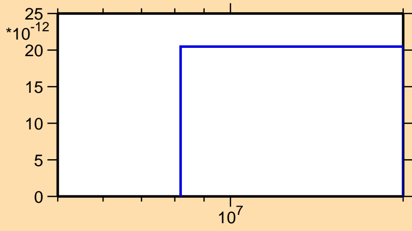
\sigma vs. E for ^{98}\text{Mo}(n,\text{He3})
