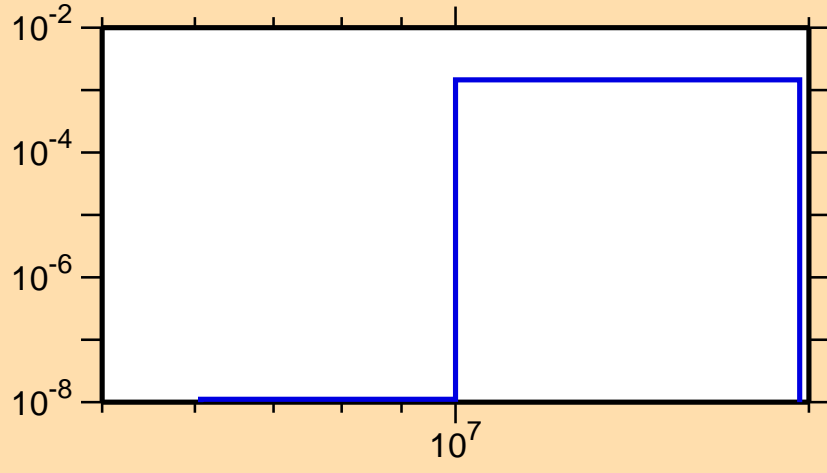
\sigma vs. E for ^{99}\text{Mo}(n,n\alpha)
