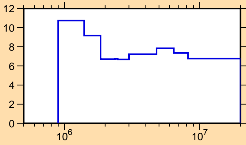
\Delta\sigma/\sigma vs. E for ^{99}\text{Mo}(n,n\text{onel.})
