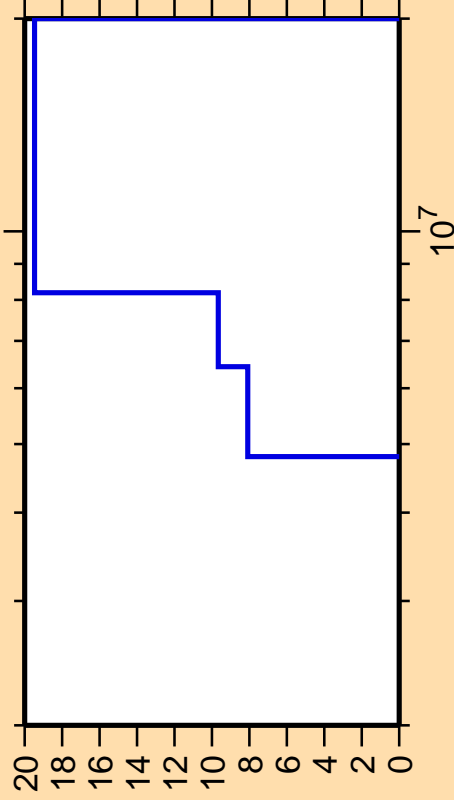
\Delta\sigma/\sigma vs. E for ^{99}\text{Mo}(n,n\text{cont.})
