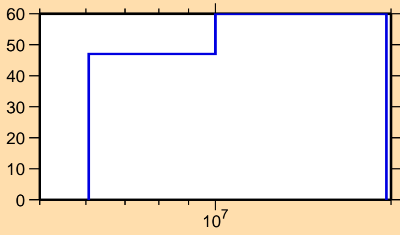
\Delta\sigma/\sigma vs. E for ^{100}\text{Mo}(n,\gamma)
