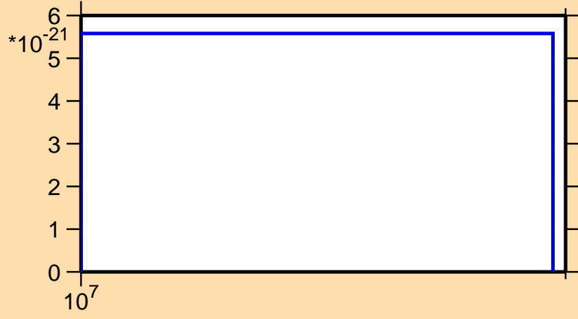
\sigma vs. E for ^{100}\text{Mo} (mt 34)
