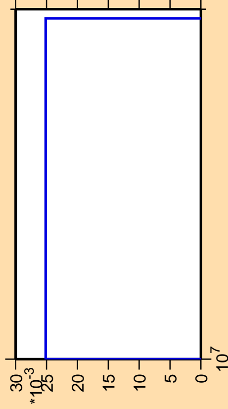
\Delta\sigma/\sigma vs. E for ^{100}\text{Mo}(n,\text{He}3)
