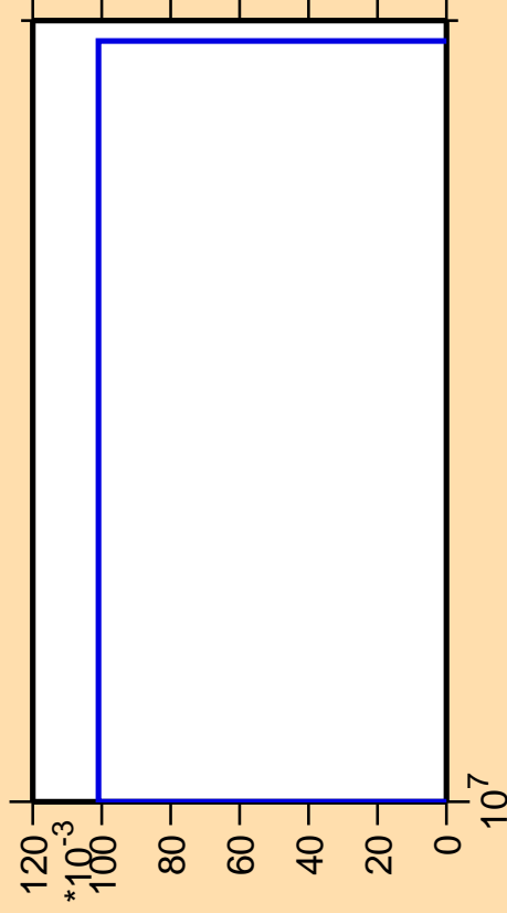
\Delta\sigma/\sigma vs. E for ^{100}\text{Mo}(n,2np)
