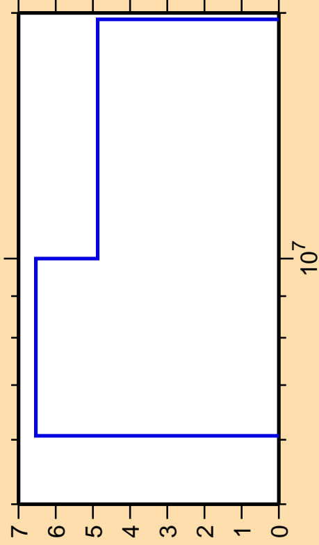
\Delta\sigma/\sigma vs. E for ^{100}\text{Mo}(n,2n)
