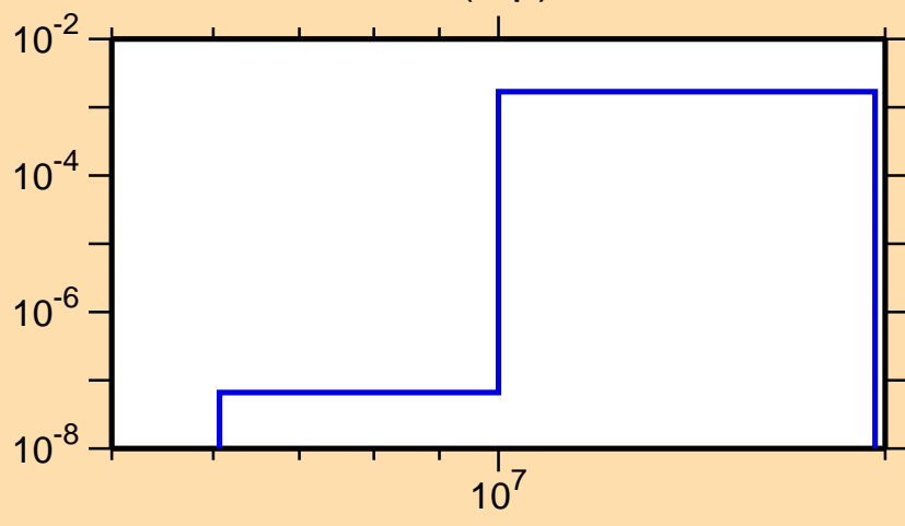
\sigma vs. E for ^{100}\text{Mo}(n,p)
