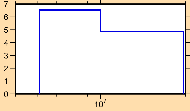
\Delta\sigma/\sigma vs. E for ^{100}\text{Mo}(n,2n)
