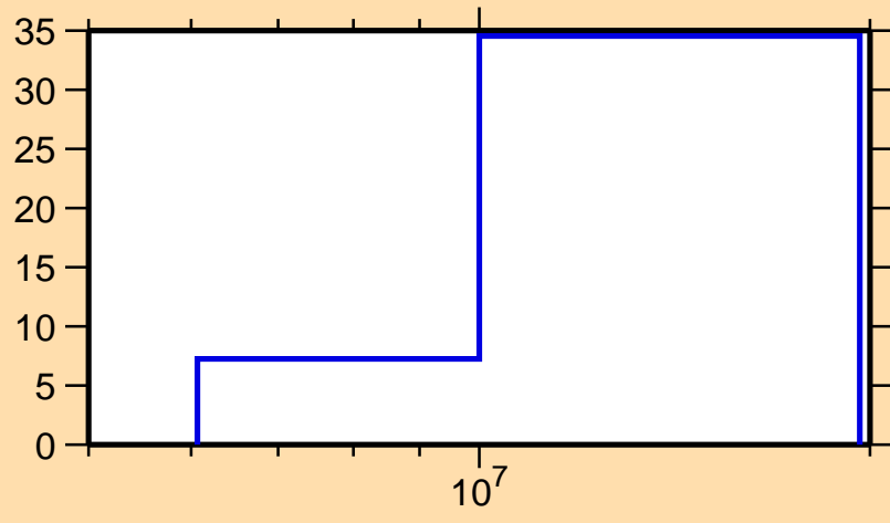
\Delta\sigma/\sigma vs. E for ^{100}\text{Mo}(n,ncont.)
