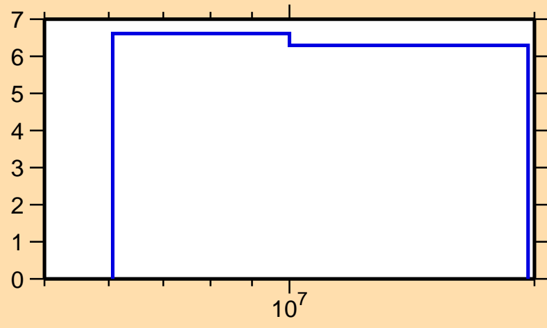
\Delta\sigma/\sigma vs. E for ^{100}\text{Mo}(n,\text{el.})
