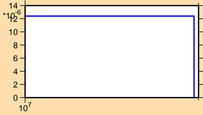
\sigma vs. E for ^{100}\text{Mo}(n,t)
