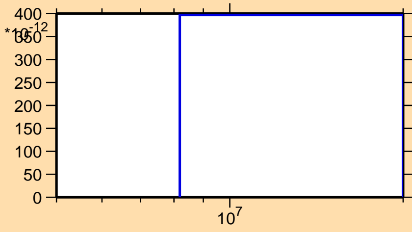
\sigma vs. E for ^{100}\text{Mo}(n,2n\alpha)
