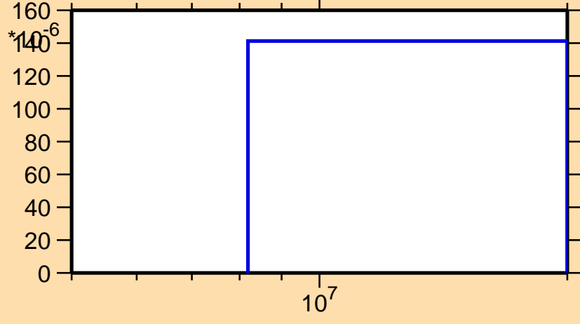
\sigma vs. E for ^{100}\text{Mo}(n,d)
