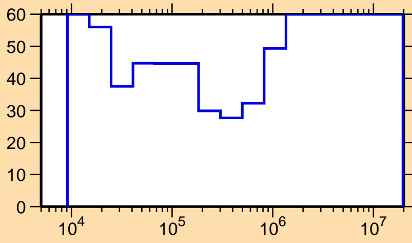
\Delta\sigma/\sigma vs. E for ^{101}\text{Mo}(n,n_1)
