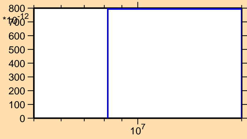
\sigma vs. E for ^{101}\text{Mo}(n,nt)
