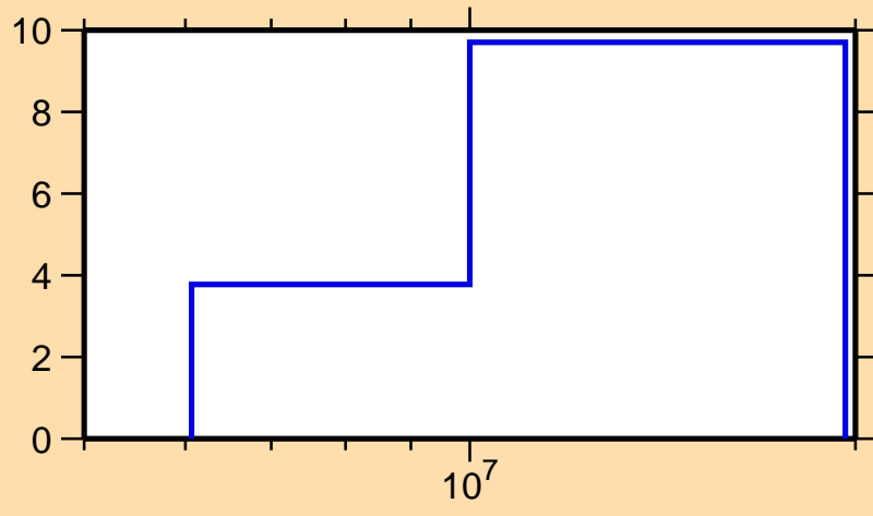
\Delta\sigma/\sigma vs. E for ^{102}\text{Mo}(n,2n)
