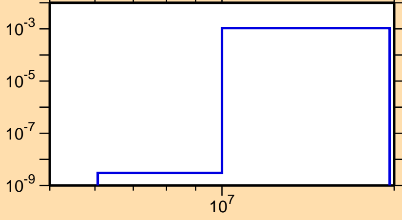
\sigma vs. E for ^{102}\text{Mo}(n,p)
