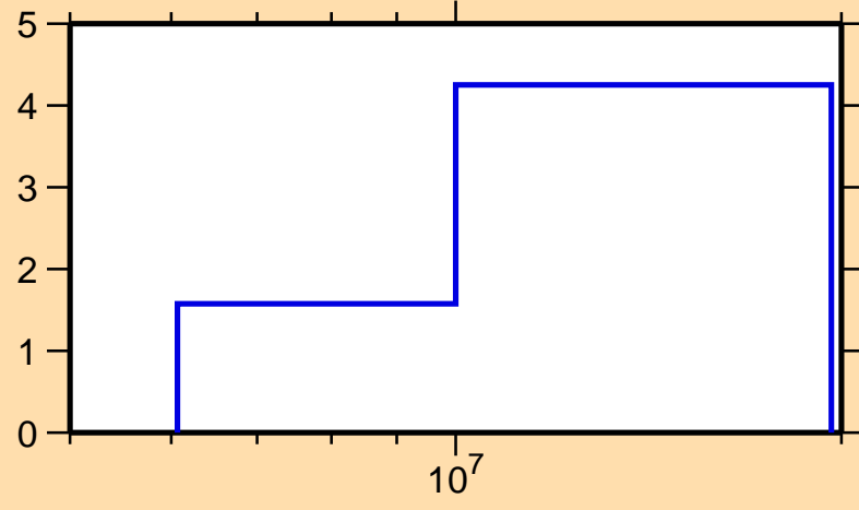
\Delta\sigma/\sigma vs. E for ^{102}\text{Mo}(n,\text{tot.})
