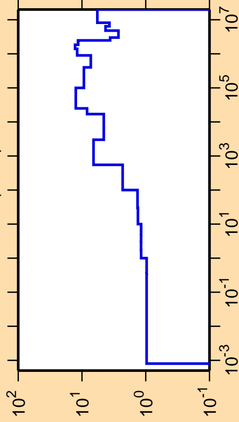
\Delta\sigma/\sigma vs. E for ^{102}\text{Mo}(n,\text{el.})
