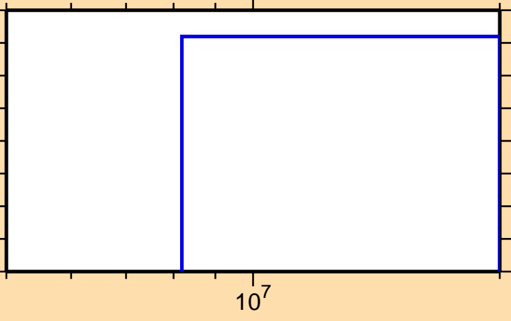
\sigma vs. E for ^{102}\text{Mo}(n,nt)
