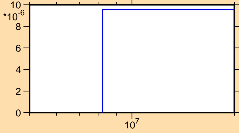
\sigma vs. E for ^{102}\text{Mo}(n,n\alpha)
