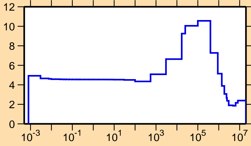
\sigma vs. E for ^{102}\text{Mo}(n,\text{el.})
