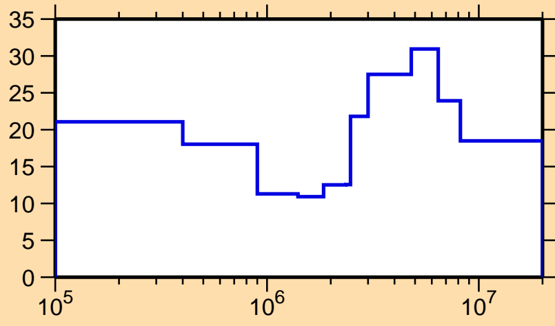
\Delta\sigma/\sigma vs. E for ^{102}\text{Mo}(n,n_1)
