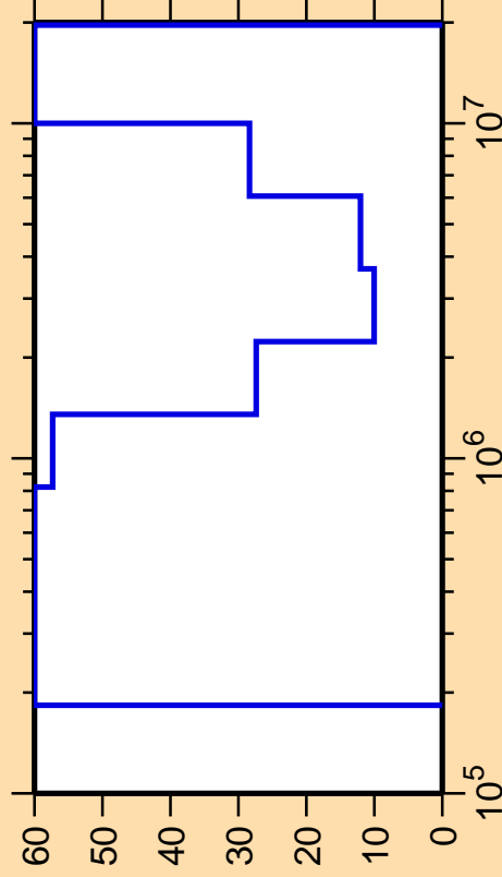
\Delta\sigma/\sigma vs. E for ^{104}\text{Mo}(n,\text{inel.})
