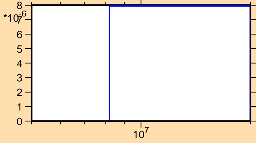
\sigma vs. E for ^{104}\text{Mo}(n,d)
