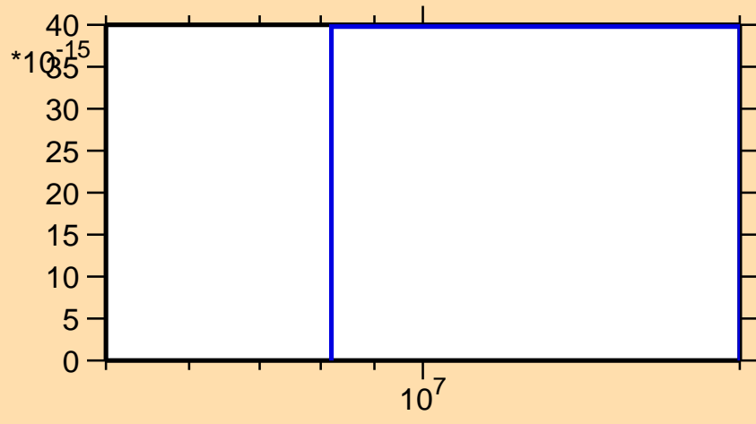
\sigma vs. E for ^{104}\text{Mo}(n,2n\alpha)
