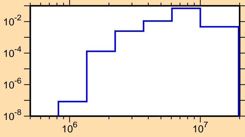
\sigma vs. E for ^{105}\text{Mo}(n,n\text{cont.})
