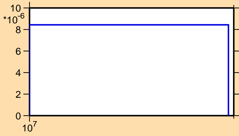
\sigma vs. E for ^{105}\text{Mo}(n,d)
