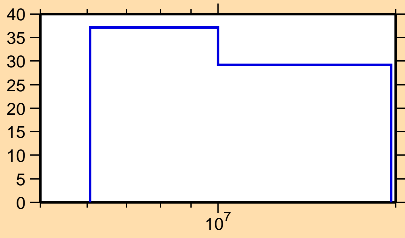
\Delta\sigma/\sigma vs. E for ^{105}\text{Mo}(n,n_1)
