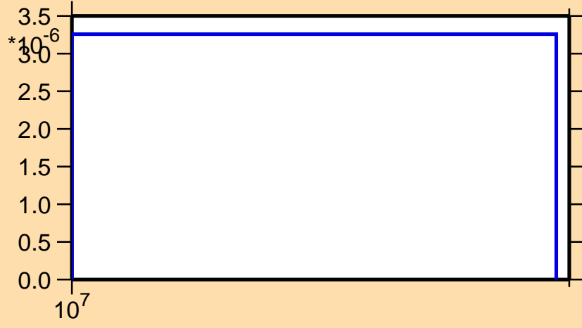
\sigma vs. E for ^{105}\text{Mo}(n,t)
