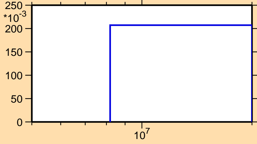
\sigma vs. E for ^{105}\text{Mo}(n,3n)
