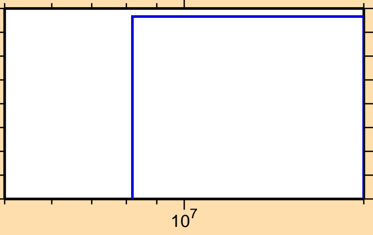
\sigma vs. E for ^{105}\text{Mo}(n,\text{nd})
