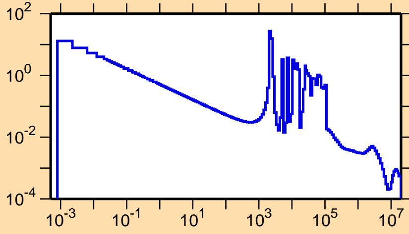
\sigma vs. E for ^{106}\text{Mo}(n,\gamma)
