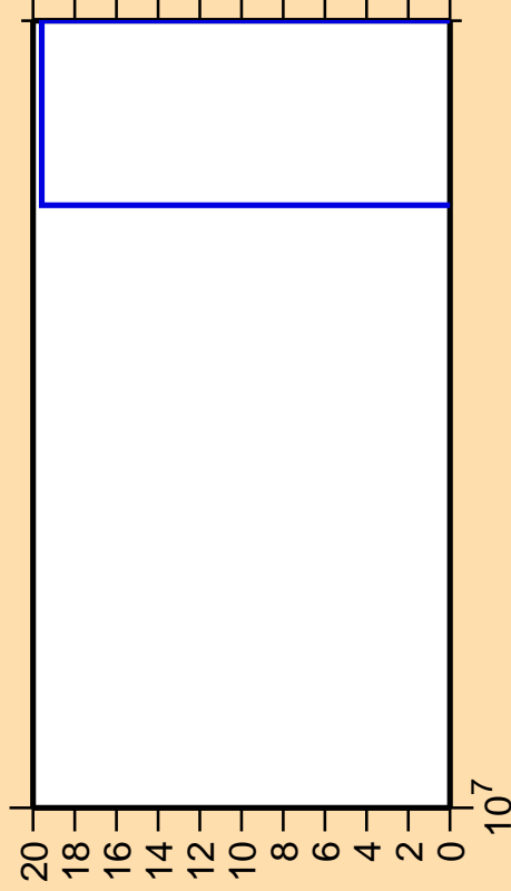
\Delta\sigma/\sigma vs. E for ^{106}\text{Mo}(n,nd)
