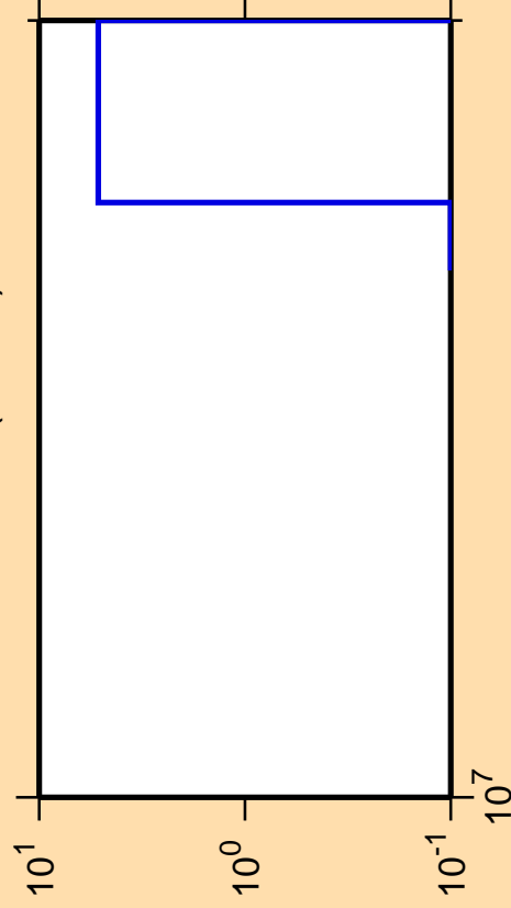
\Delta\sigma/\sigma vs. E for ^{106}\text{Mo}(n,2n\alpha)
