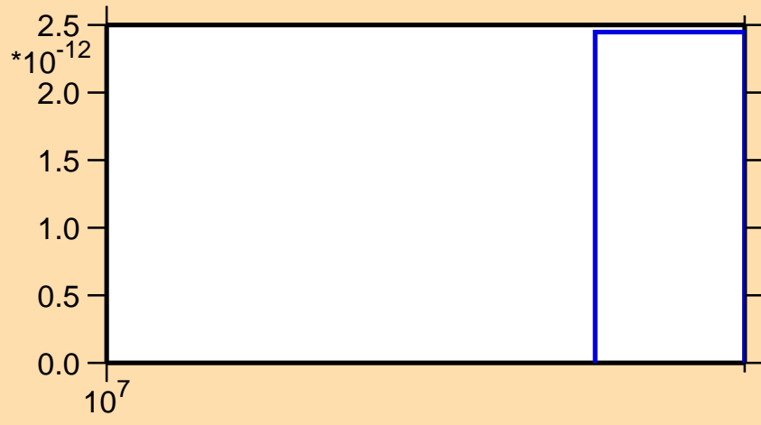
\sigma vs. E for ^{106}\text{Mo}(n,nd)
