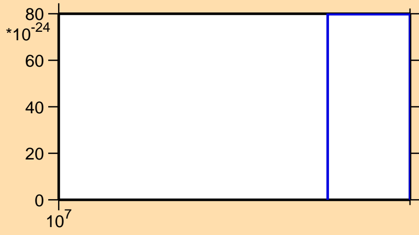
\sigma vs. E for ^{106}\text{Mo}(n,2np)
