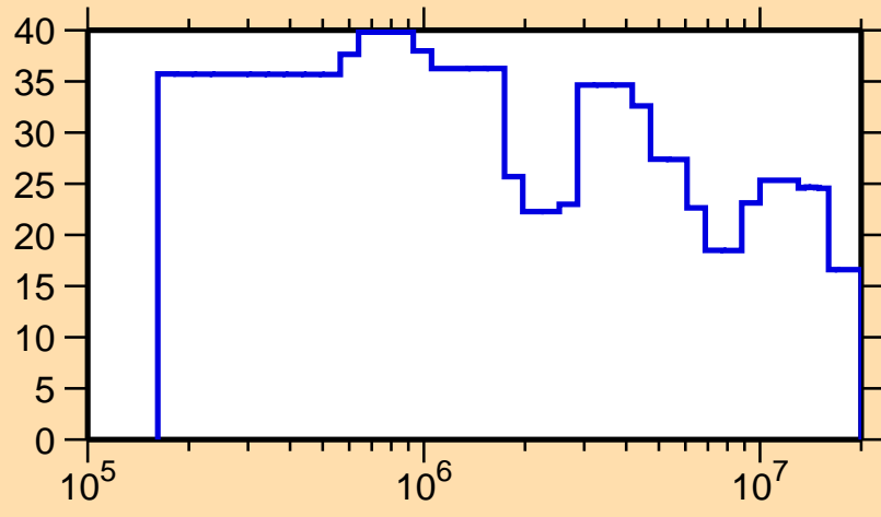
\Delta\sigma/\sigma vs. E for ^{106}\text{Mo}(n,\text{el.})
