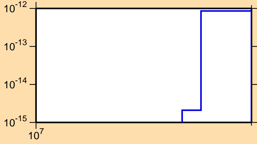
\sigma vs. E for ^{106}\text{Mo}(n,2n\alpha)
