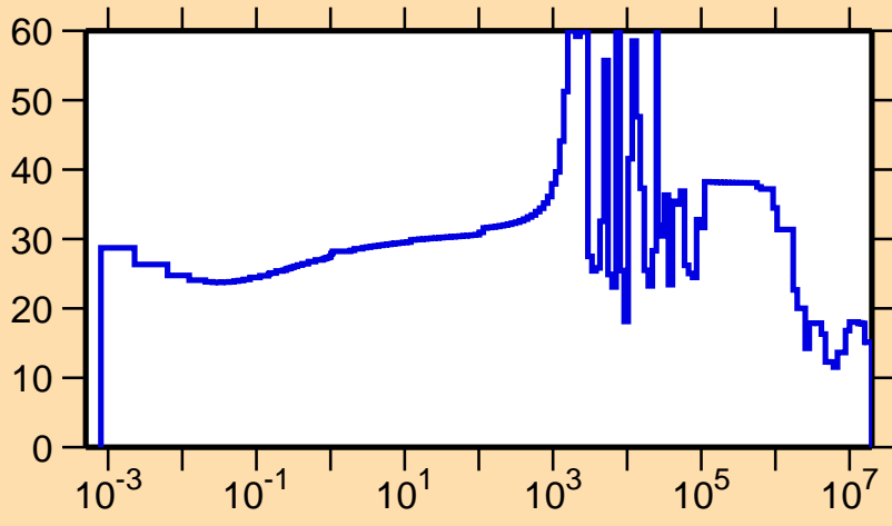
\Delta\sigma/\sigma vs. E for ^{106}\text{Mo}(n,\text{tot.})
