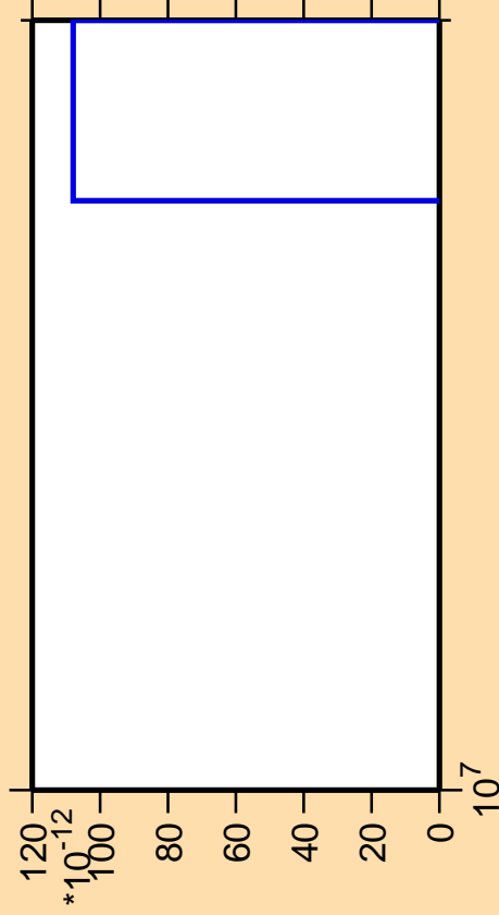
\Delta\sigma/\sigma vs. E for ^{106}\text{Mo}(n,2np)
