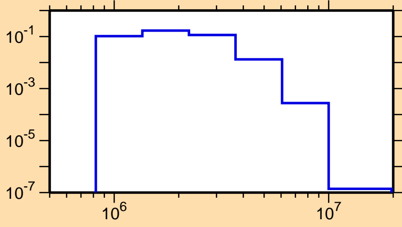
\sigma vs. E for ^{106}\text{Mo}(n,n_4)
