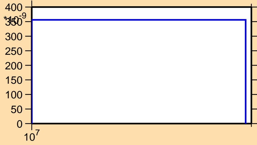
\sigma vs. E for ^{106}\text{Mo}(n,np)
