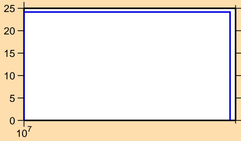
\Delta\sigma/\sigma vs. E for ^{106}\text{Mo}(n,el.)
