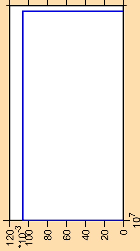
\Delta\sigma/\sigma vs. E for ^{106}\text{Mo}(n,\text{nd})
