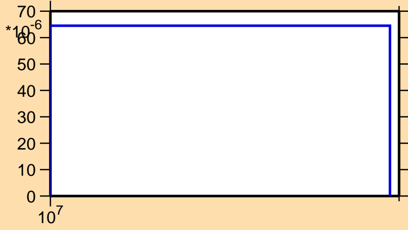
\sigma vs. E for ^{106}\text{Mo}(n,p)
