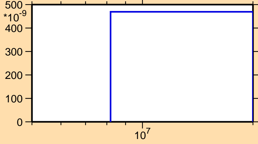
\sigma vs. E for ^{106}\text{Mo}(n,t)
