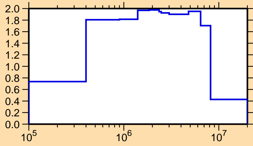
\sigma vs. E for ^{106}\text{Mo}(n,\text{inel.})
