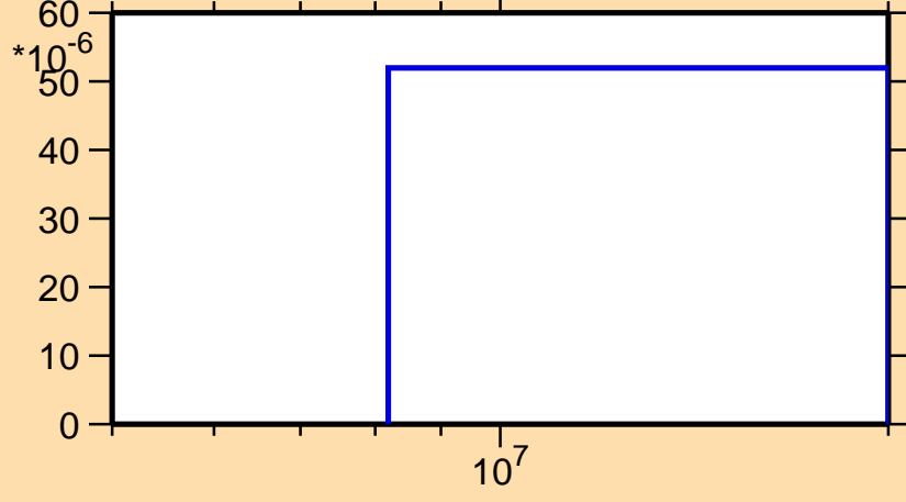
\sigma vs. E for ^{106}\text{Mo}(n,p)
