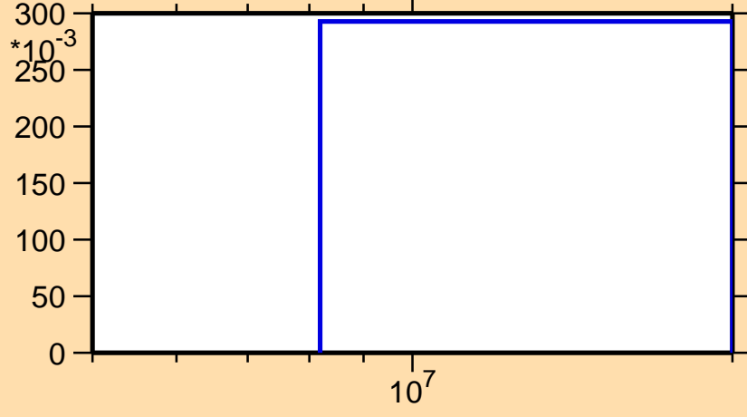
\sigma vs. E for ^{106}\text{Mo}(n,3n)
