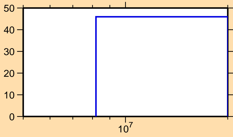
\Delta\sigma/\sigma vs. E for ^{106}\text{Mo}(n,n_1)
