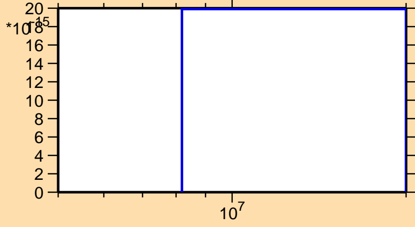
\sigma vs. E for ^{106}\text{Mo}(n,\text{nd})
