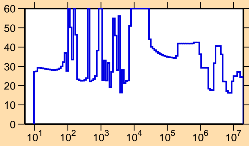
\Delta\sigma/\sigma vs. E for ^{107}\text{Mo}(n,\text{el.})
