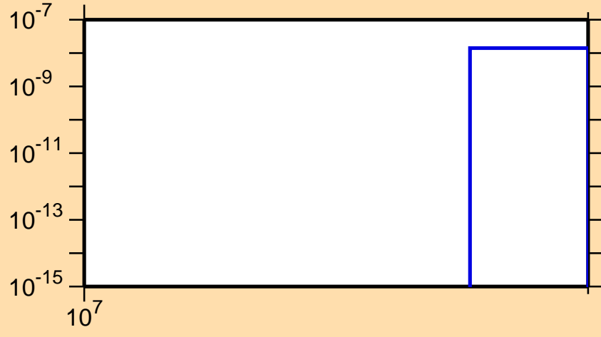
\sigma vs. E for ^{107}\text{Mo}(n,\text{nd})
