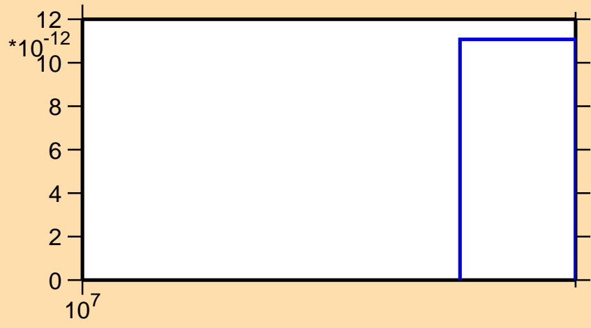
\sigma vs. E for ^{107}\text{Mo}(n,2np)
