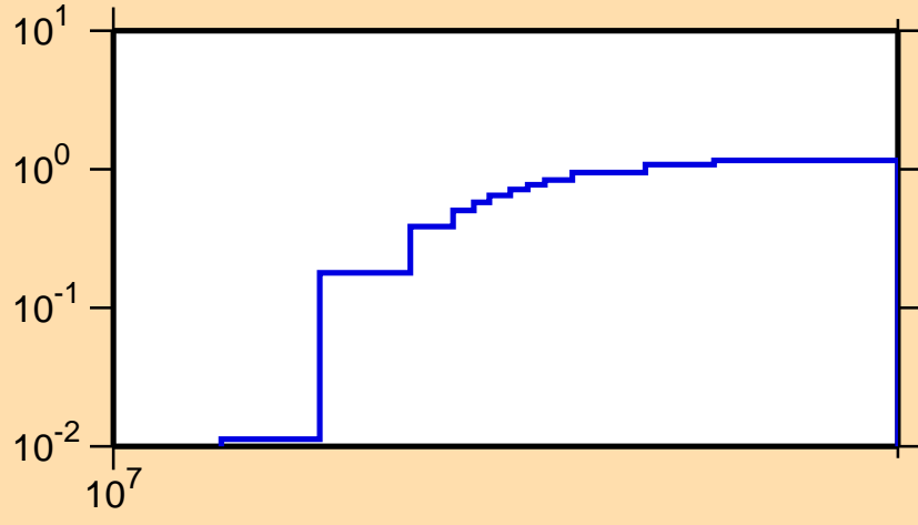
\sigma vs. E for ^{107}\text{Mo}(n,3n)
