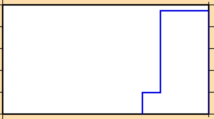
\sigma vs. E for ^{107}\text{Mo}(n,2n\alpha)
