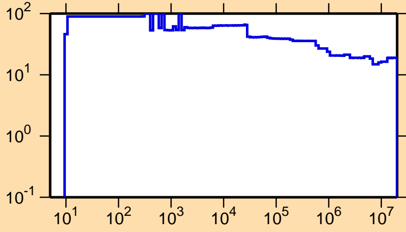
\Delta\sigma/\sigma vs. E for ^{107}\text{Mo}(n,\text{nonel.})
