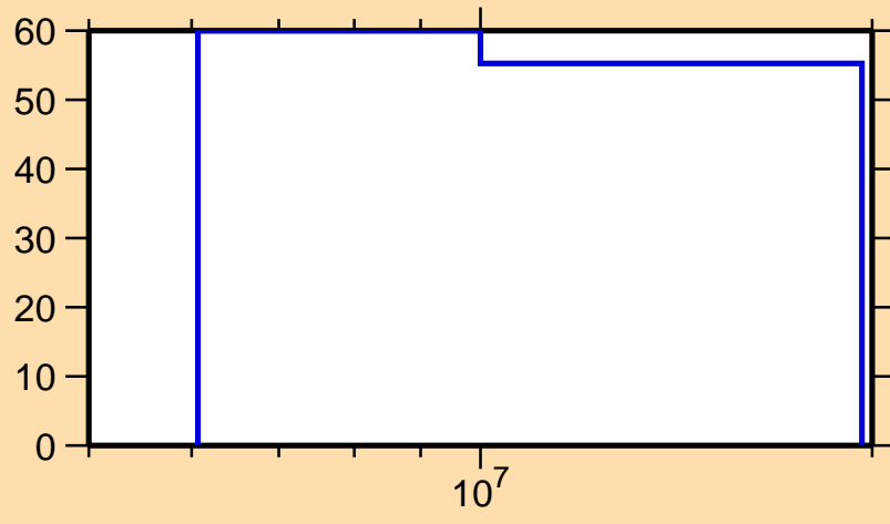
\Delta\sigma/\sigma vs. E for ^{107}\text{Mo}(n,n_1)
