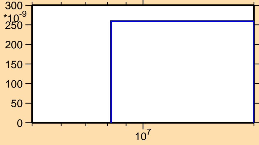
\sigma vs. E for ^{107}\text{Mo}(n,n\alpha)
