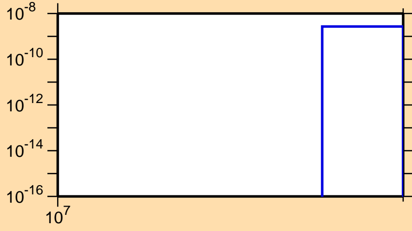
\sigma vs. E for ^{108}\text{Mo}(n,nt)
