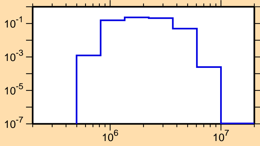
\sigma vs. E for ^{108}\text{Mo}(n,n_4)
