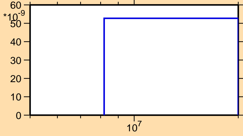
\sigma vs. E for ^{108}\text{Mo}(n,np)
