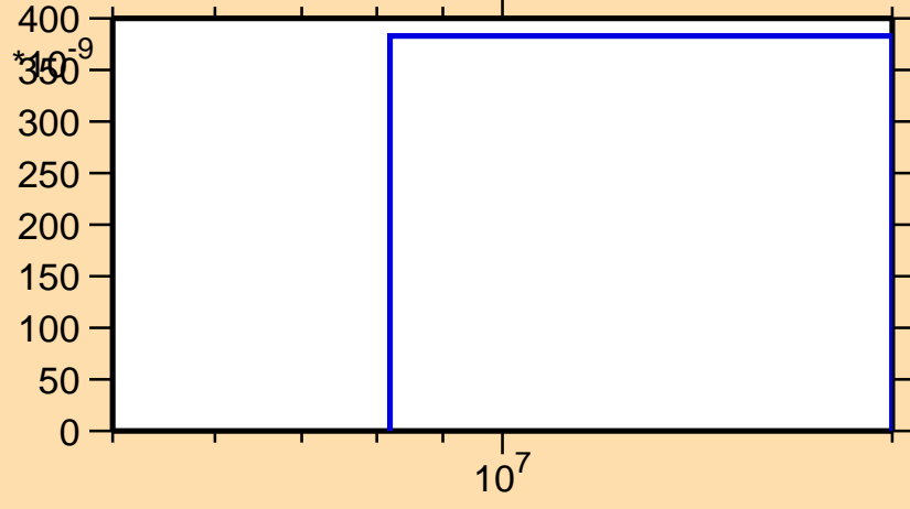
\sigma vs. E for ^{108}\text{Mo}(n,d)
