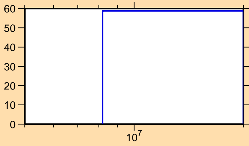
\Delta\sigma/\sigma vs. E for ^{108}\text{Mo}(n,ncont.)
