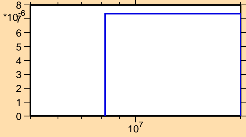
\sigma vs. E for ^{108}\text{Mo}(n,p)
