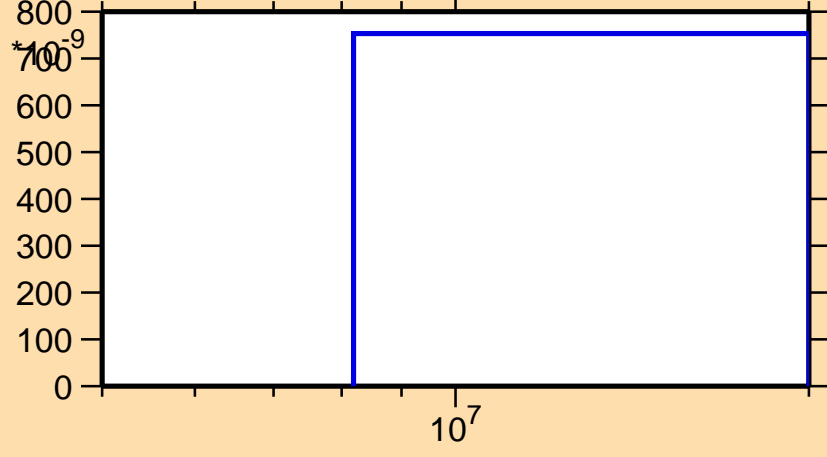
\sigma vs. E for ^{108}\text{Mo}(n,\alpha)
