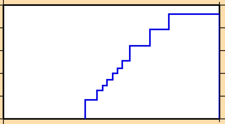
\sigma vs. E for ^{277}
