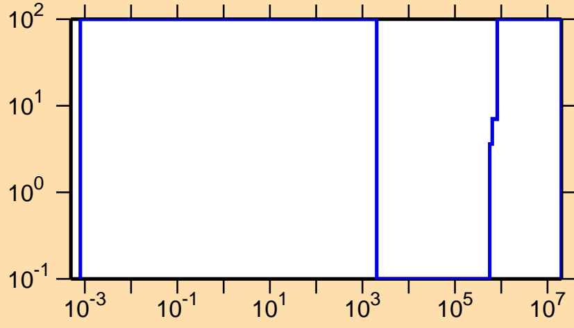
\Delta\sigma/\sigma vs. E for ^{278}\gamma
