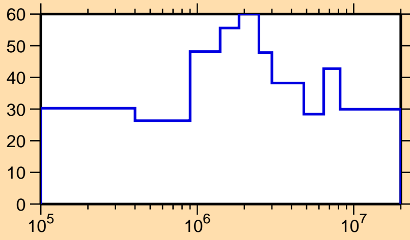
\Delta\sigma/\sigma vs. E for ^{278}_1
