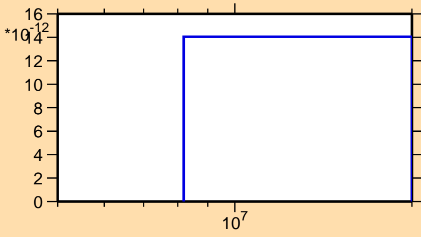
\sigma vs. E for ^{278}\text{He3}
