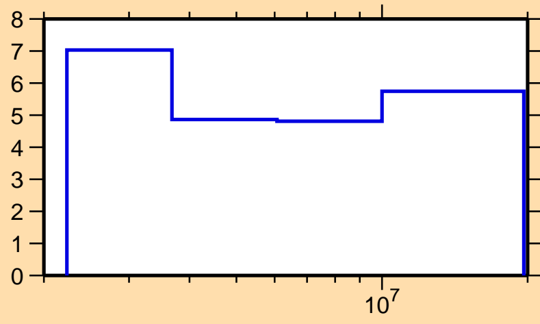
\Delta\sigma/\sigma vs. E for ^{279}
