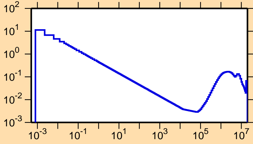
\sigma vs. E for ^{13}\text{N}(n,d)
