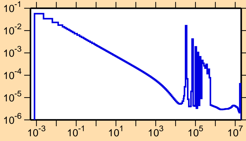
\sigma vs. E for ^{13}\text{N}(n,\gamma)
