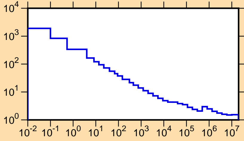
\sigma vs. E for ^{13}\text{N}(n,\text{tot.})
