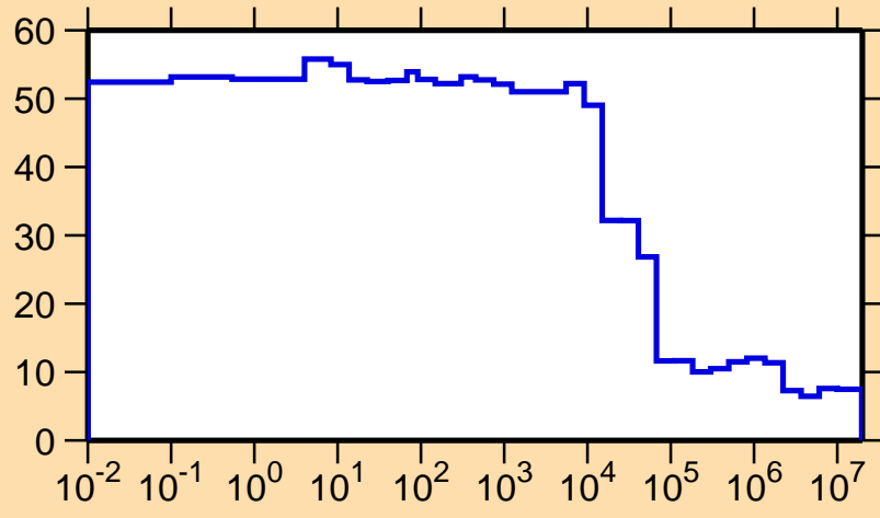
\Delta\sigma/\sigma vs. E for ^{13}\text{N}(n,\text{nonel.})
