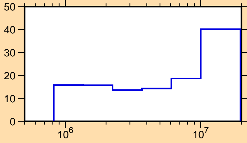
\Delta\sigma/\sigma vs. E for ^{13}\text{N}(n,p)
